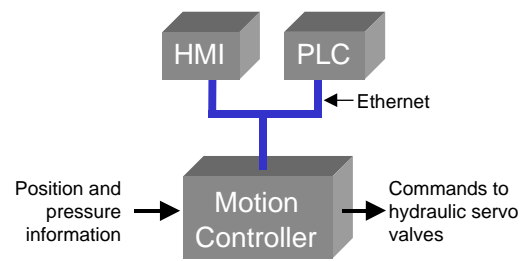
Figure 1. Modular control system based on Ethernet.
